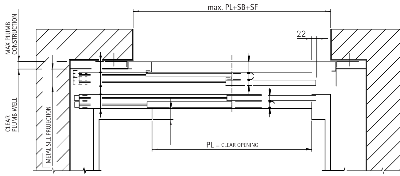
NICHE INSTALLATION
